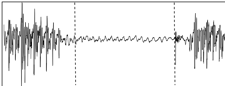
Figure 4.8. Waveform illustrating the sequence /p-d/ realized as [b-d]. Word: daydodá̌p-dá̌p ‘armadillo, sp.’ (EM)
