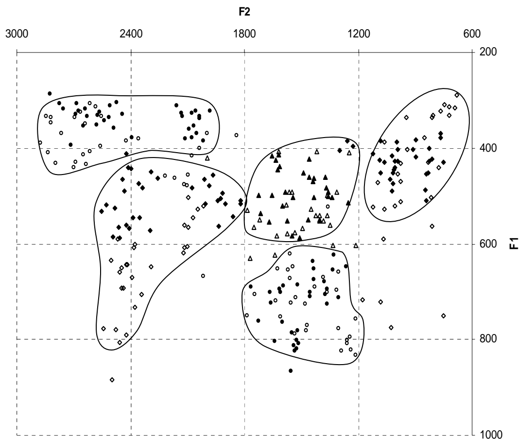
Figure 2.3. F1 vs. F2 plots of Mundurukú oral-nasal vowels. In each pair of vowels, black stands for oral vowels and white for nasal vowels. Speakers: AK, JT and EM (Average of 29 tokens for each vowel)
