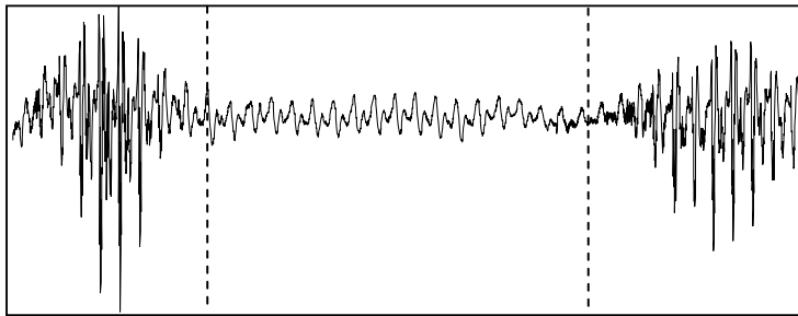
Figure 4.7. Waveform illustrating the sequence /k-ɕ/ realized as [g-ɕ]. Word: aɕó̌k-ɕó̌ŋ ‘bathing’ (EM)
