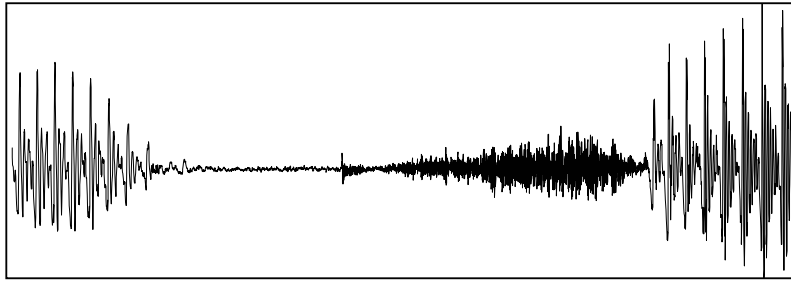
Figure 4.13. Expanded waveform illustrating the stop + fricative sequence /p-s/. Word: dápsẽm ‘deer’ (JT)
