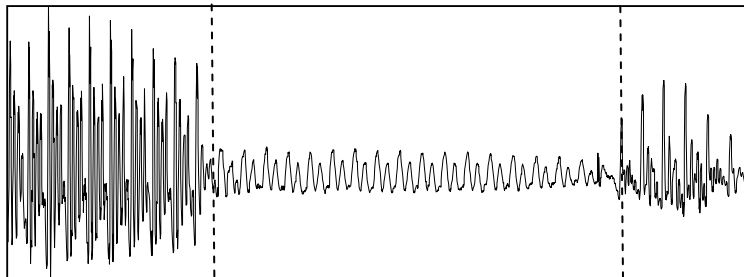
Figure 4.5. Waveform illustrating the sequence /p-b/ realized as a long [b]. Word: təp-boŋ 'The leaf is big.' (JT)
