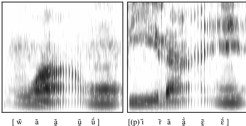
Figure 3.15. Spectrograms illustrating the sequence [ṽʔṽ] in the Mundurukú words waʔó ‘my voice, language’, and piraʔé ‘dry fish’.
