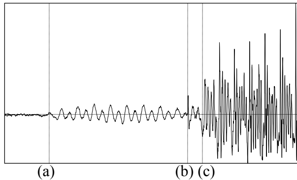
Figure 3.4. Waveform of word-initial /d/ in the Mundurukú word daŋé ‘hawk, sp.’; (a) marks the onset of prevoicing, (b) marks the onset of the burst, and (c) the offset of the burst and beginning of the vowel.
