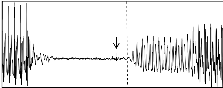
Figure 4.14. Expanded waveform of the sequence /t-m/. Word: otomóŋ ‘I put the bunch.’ (JT)
