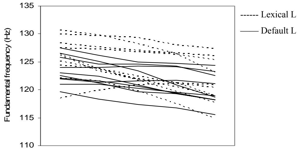
Figure 8.3. Graph showing F0 realization for default and lexical L-tones in two sequences /ɖʒe/ in the Mundurukú words daɖʒebáró ‘porcine’ and waɖʒebá ‘cocoa’. (AK; ten tokens for each tone).
