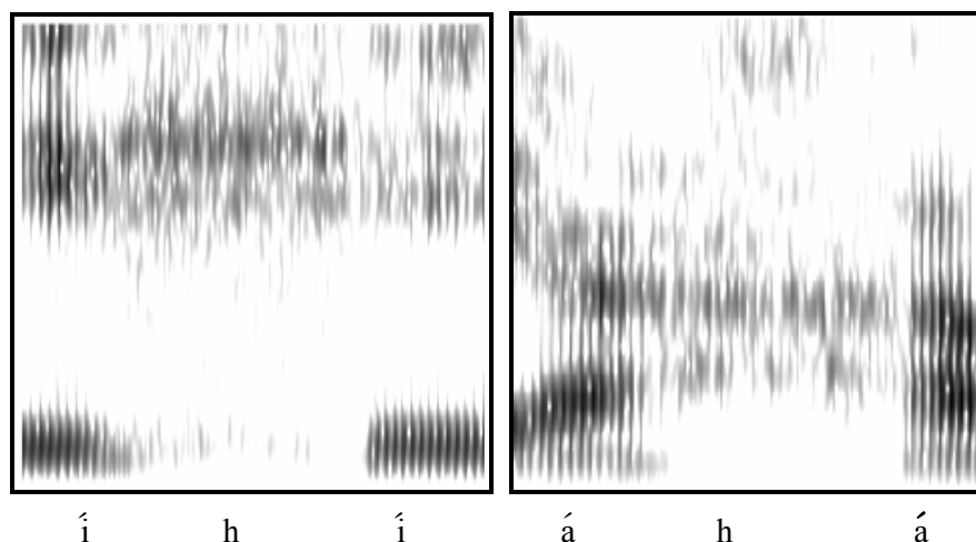
Figure 6.1. Spectrograms of VhV sequences in the Mundurukú words íhí ‘winter’ and iáhám ‘to bite s.t.’.
