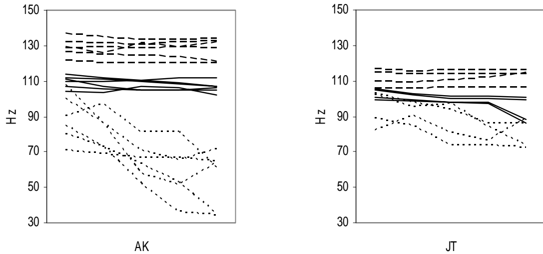
Figure 2.10. Graphs showing F0 realization for H-tone, L-tone and creaky vowels. Dashed lines are for H-tone /ó/, solid lines for L-tone /o/, and dotted lines for creaky voice /ǒ/.
