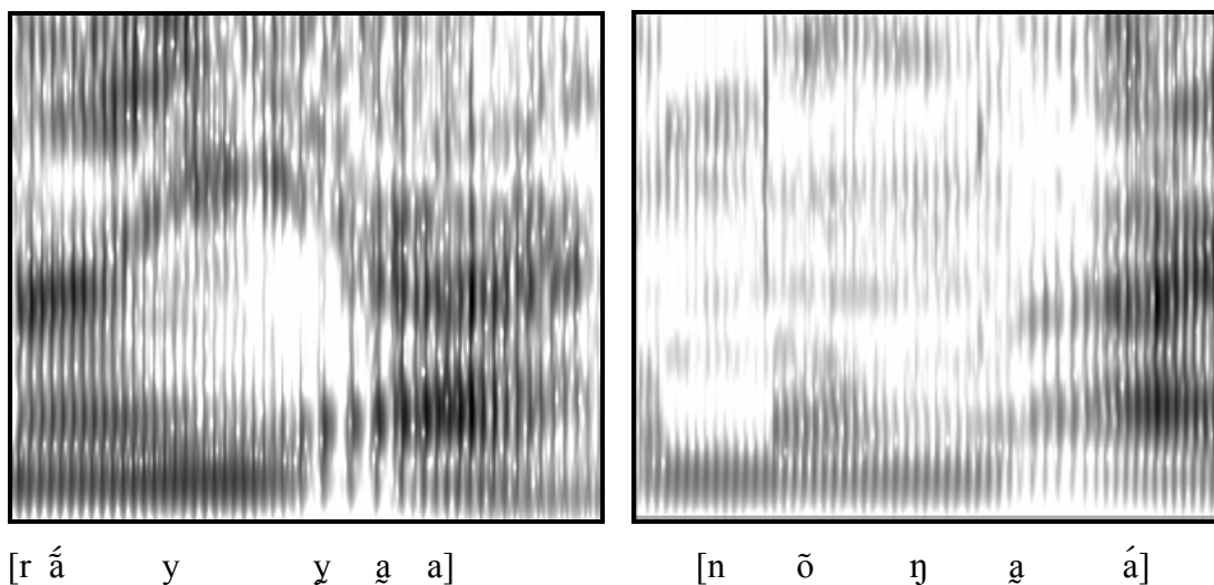
Figure 3.14. Spectrograms showing /ʔ/ after a glide and a nasal consonant. The spectrogram in the left shows only the underlined part of the word ʕaráyʔa ‘orange’, and the second spectrogram shows the entire word nōŋʔá ‘flea’.
