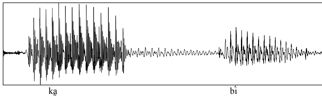
Figure 8.8. Waveform of the Mundurukú word kəbí ‘sky’. (JT)
