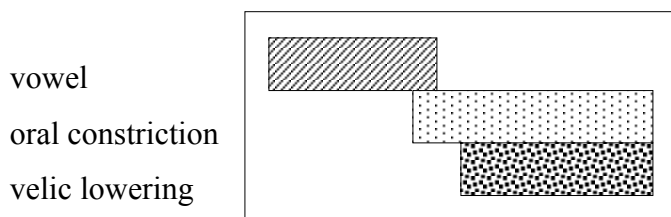
Figure 3.7. Schematic representation of the relative timing of velic and oral gestures in preoralized nasals.
