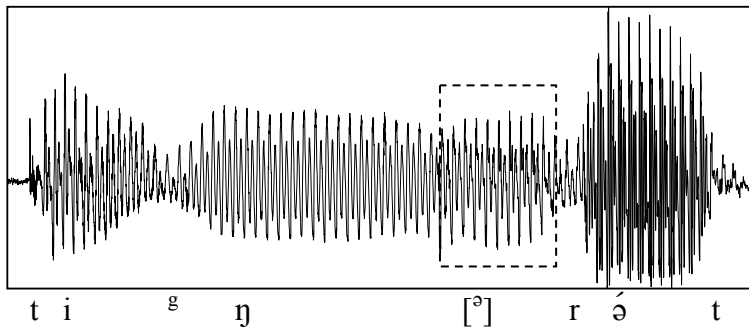
Figure 4.19. Waveform illustrating non-syllabic [ə] in nasal + /r/. Word: tiŋrət ‘The smoke is white.’ (JT)
