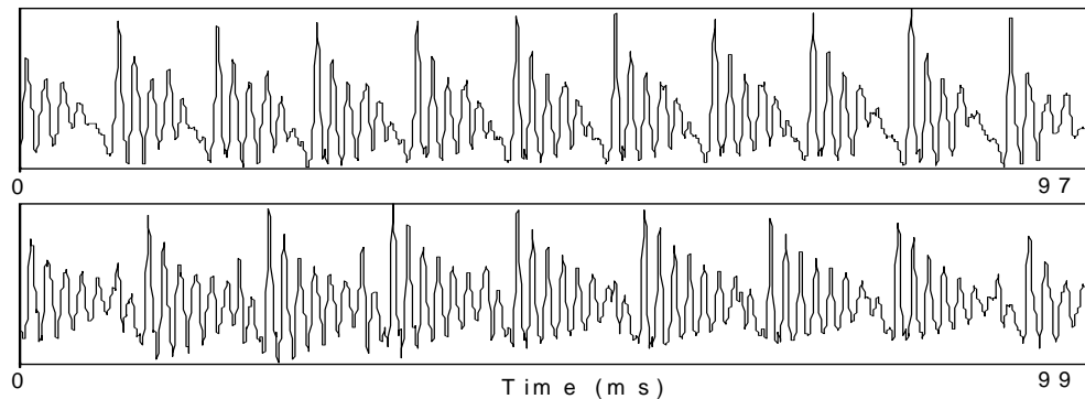
Figure 2.4. Waveforms illustrating modal [a] and creaky [a]. Words: dat ‘scorpion’ and dat ‘vomit’, respectively.
