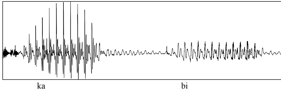
Figure 8.9. Waveform of the noun kabi ‘sky’ in the Mundurukú word kabi-diŋ ‘mist’. (JT)
