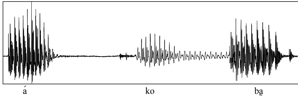
Figure 8.6. Waveform showing a creaky vowel in the Mundurukú word áko-bɔ ‘banana’. (JT)
