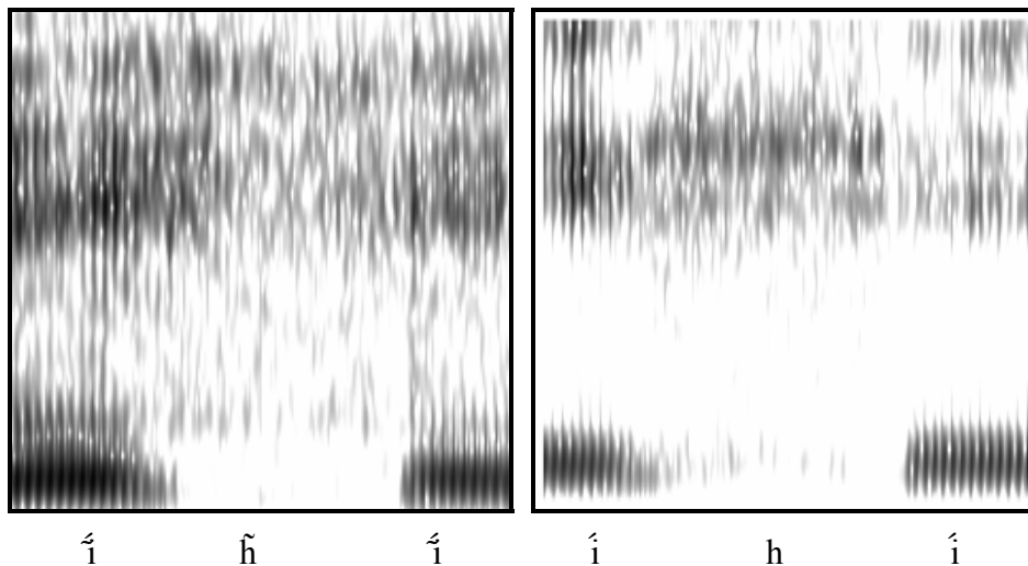
Figure 3.9. Spectrograms of [ṽh̃ṽ] and [vhv] sequences in the Mundurukú words íhí ‘winter’ and áihĩ ‘mother, Voc.’.
