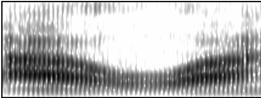
Figure 4.2. Spectrogram showing an intervocalic [w] in the Mundurukú word áwá ‘grandmother’.
