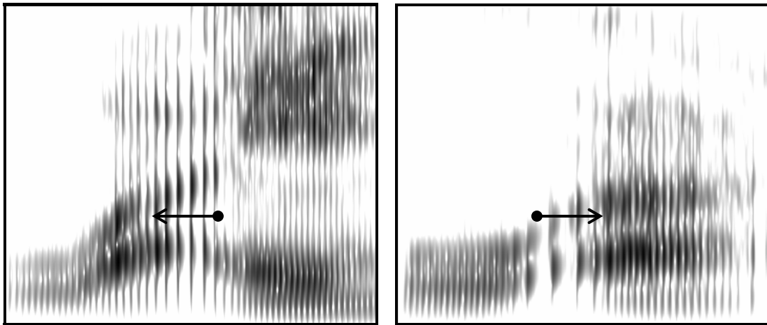
Figure 3.12. Spectrograms illustrating the realization of an intervocalic /ʔ/. The spectrogram on the left is a sample of the word waʔé ‘bowl’, and on the right a sample of the word óʔa ‘axe’.
