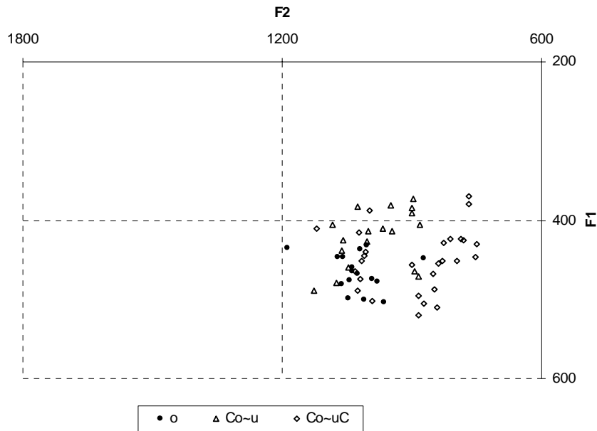
Figure 2.2. A comparison between [o] and [o~u]. Words okpot ‘my son (male speech)’, itop ‘her husband’, iməpók ‘to beat s.o. up’, irore ‘It’s loose’ and aró ‘parrot’. (Legend: “o” = nonalternating [o] (16 tokens), “Co~u” = [o~u] alternation in an open syllable (18 tokens), and “Co~uC” = [o~u] alternation in a closed syllable (14 tokens))
