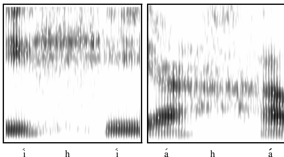
Figure 3.8. Spectrograms of VhV sequences in the Mundurukú words íhí ‘winter’ (left), and iahám ‘to go up’ (right).
