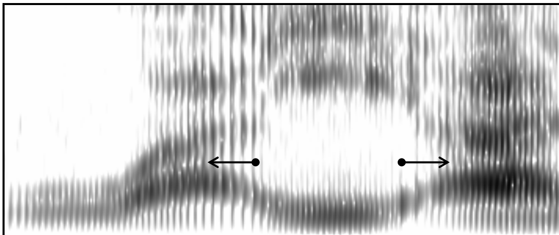
Figure 3.13. Spectrogram of the Mundurukú word waʔáʔa ‘gourd’.
