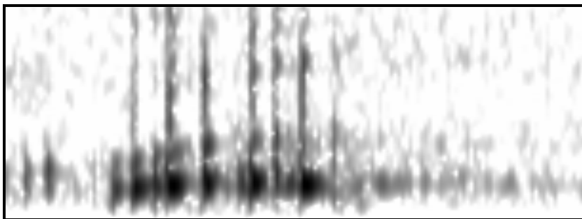
Figure 4.3. Spectrogram of the sequence /koǣ/ [k w ǣ] in the word /koqtó/ ‘summer’.
