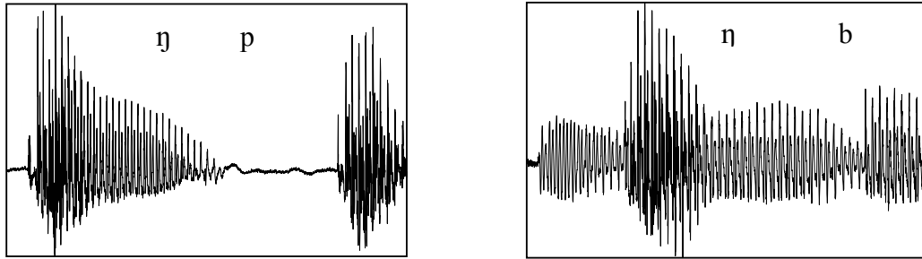
Figure 4.17. Waveforms illustrating sequences nasal + stop. Words: pə́ŋpə́ ‘one finger’ (on the left) and bə́ŋbi(wá) ‘bracelet’ (on the right). (JT)
