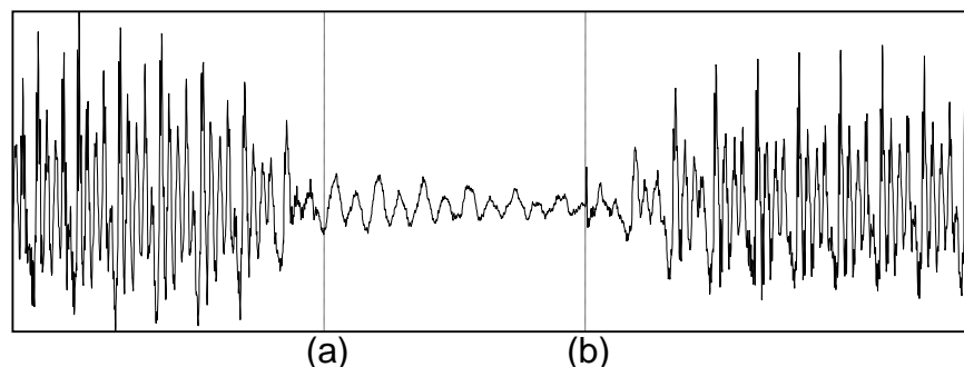
Figure 3.5. Waveform of the Mundurukú word ɕededem [ɕɛ̀ɛ̀dɛ̀dɛ̀ b m] ‘to talk’.
