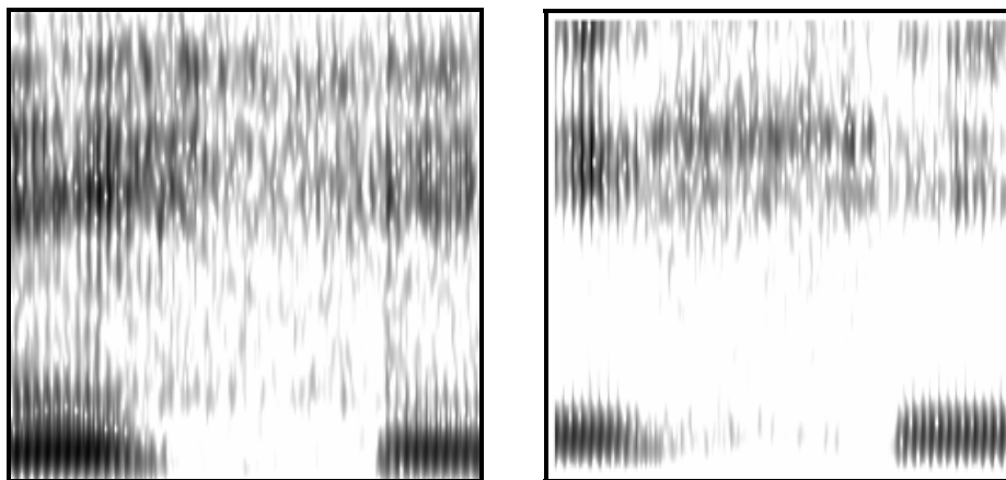
Figure 6.2. Spectrograms of VhV sequences in the Mundurukú words aĩĩĩ ‘mother’ (left) and ĩĩĩ ‘winter’ (right).
