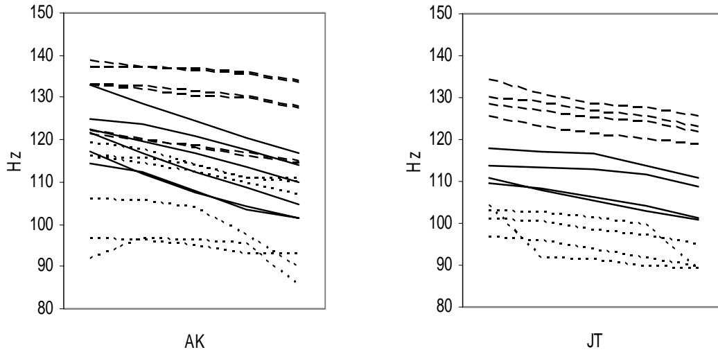
Figure 2.8. Graphs showing F0 realization for H-tone, L-tone and creaky vowels. Dashed lines are for H-tone /ǎ/, solid lines for L-tone /ǝ/, and dotted lines for creaky voice /ǽ/.
